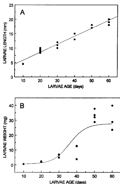
Fig. 1. A- Linear relationship ( r = 0.77 ) between total length (mm) and age (days after hatching) of sea bass ( D. labrax ) larvae from aquaculture facility. B- Relationship between total weight (mg) and age of sea bass larvae from aquaculture facility, reaching a plateau at day 50.
